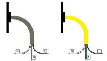
Standard Cord End
